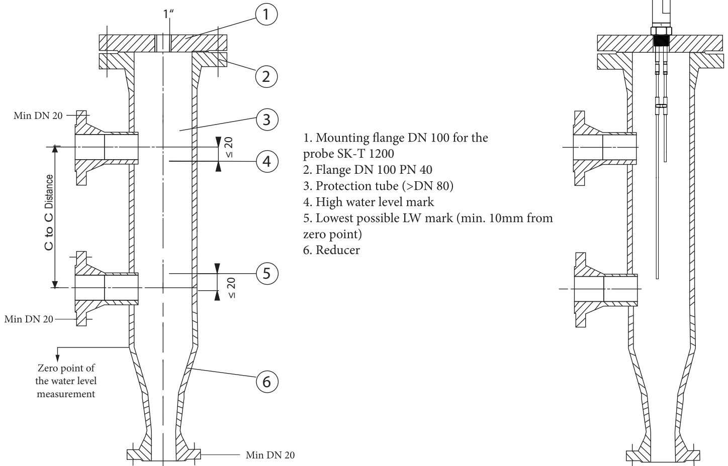
Figure 4 : Installation Example 2, Usage With Protection Tube Outside The Boiler.
